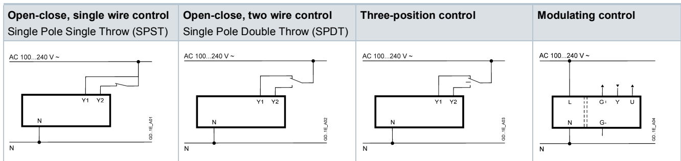
GLB3.. 1E (AC 100...240 V ~)
